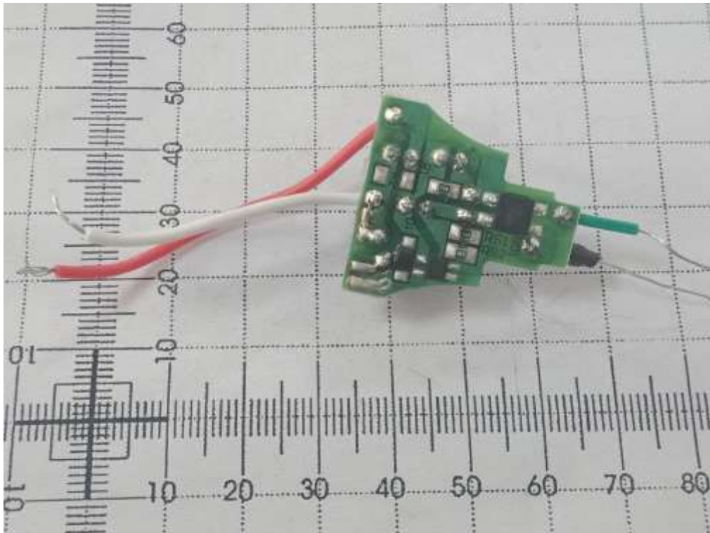
Photo 4: PCB view of G45-7-27/A12F/11
