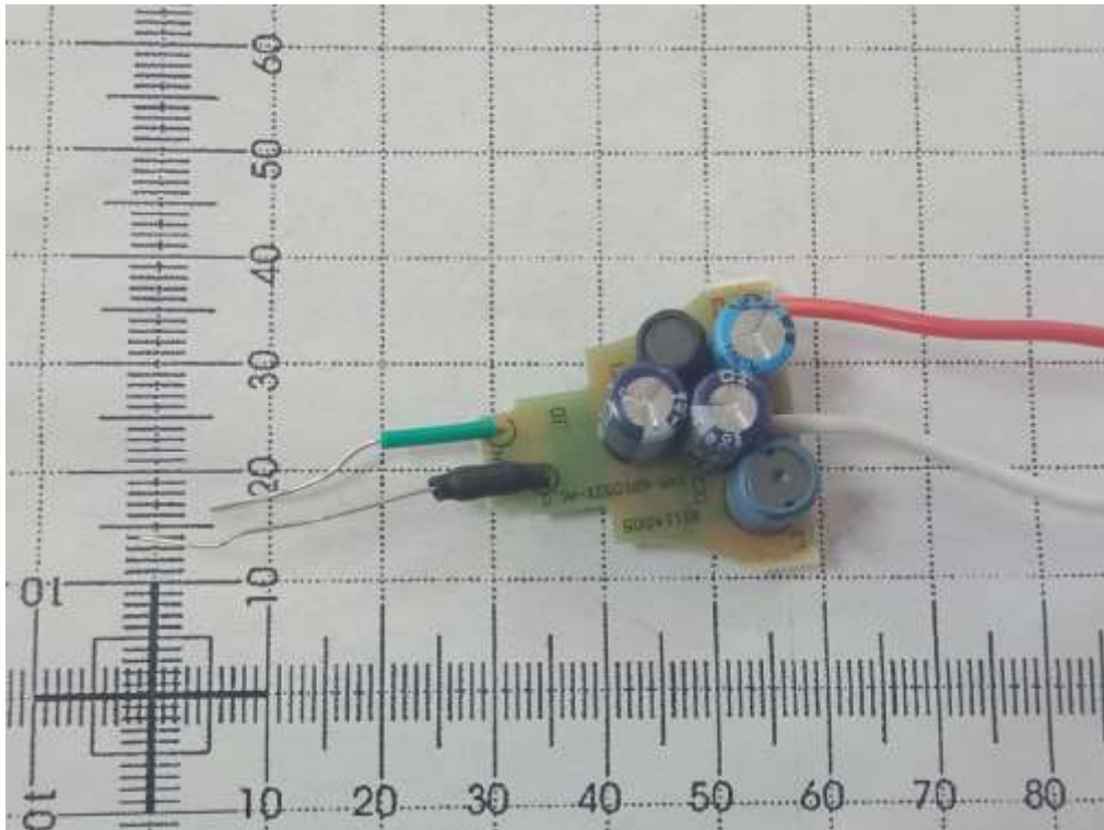
Photo 3: PCB view of G45-7-27/A12F/11
